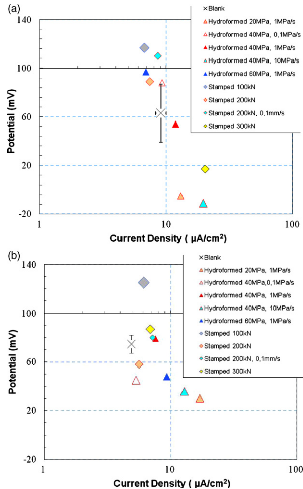
Fig. 8. Effect of pressure and stamping force on corrosion resistance with purging (a) H 2 gas, and (b) O 2 gas.
